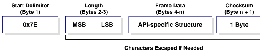
Figure 9-02. UART Data Frame Structure - with escape control characters:
